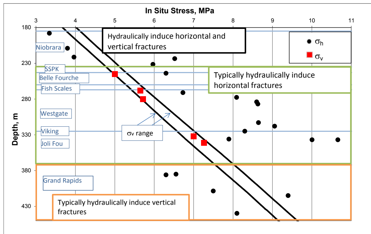
Figure 6-1 In-Situ Stresses in Primrose and Wolf Lake
