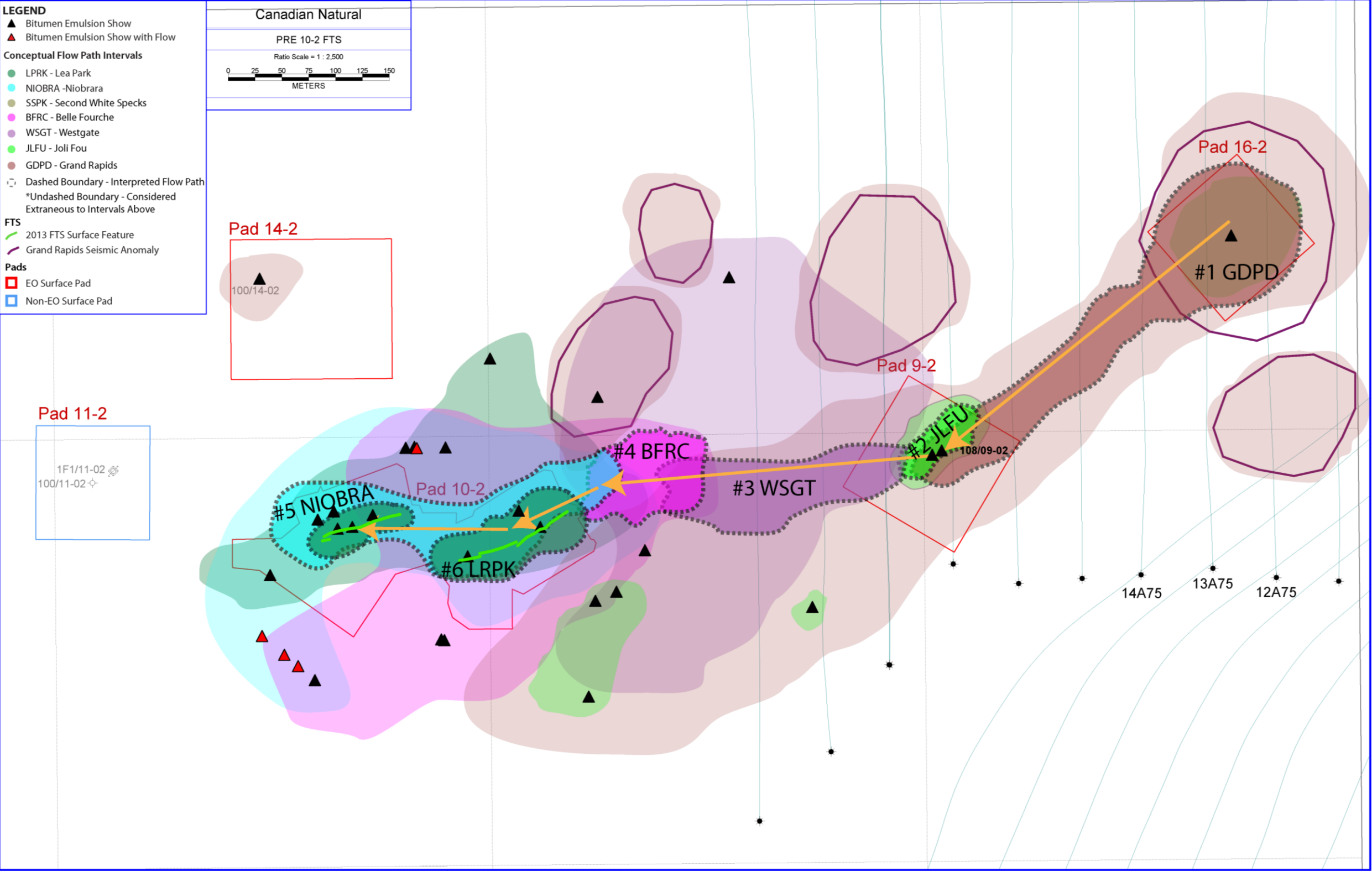
Figure 10-4 10-2 FTS – Conceptual Plan View of Bitumen Emulsion Shows
