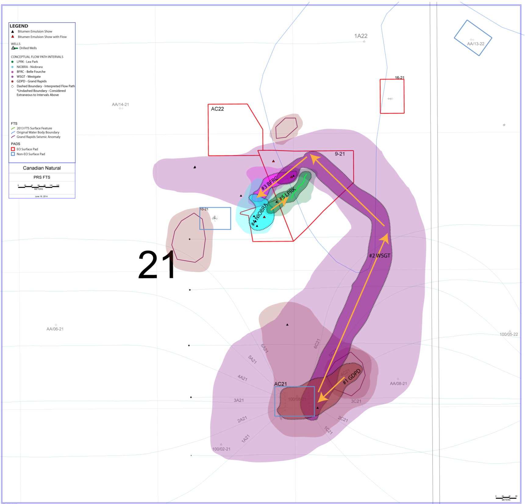
Figure 10-6 9-21 FTS – Conceptual Plan View of Bitumen Emulsion Shows
