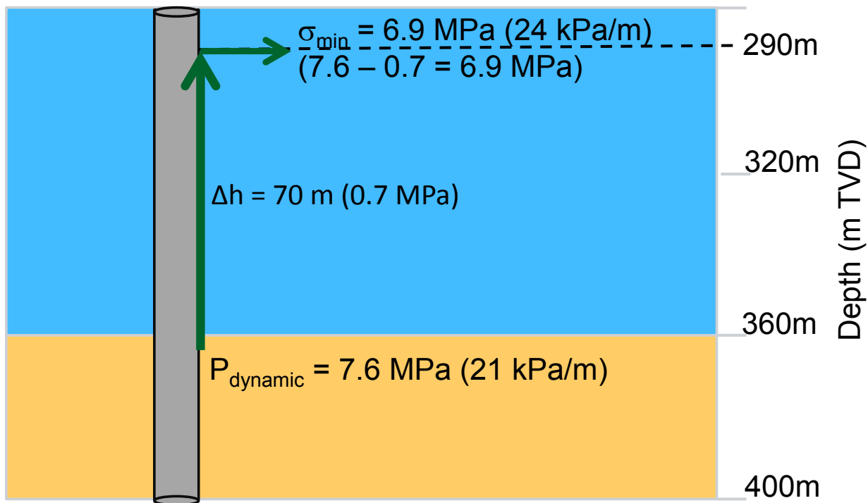
Figure 6-7 Example of pressures required for initiation of hydraulically induced fracturing in the Lower Colorado
