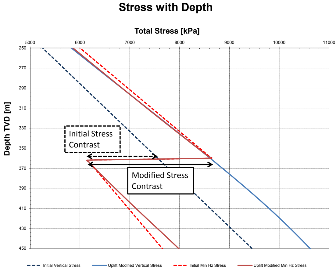
Figure 6-6 Example of calculated total stress changes with depth and effects of vertical stress approaching the minimum horizontal stress
