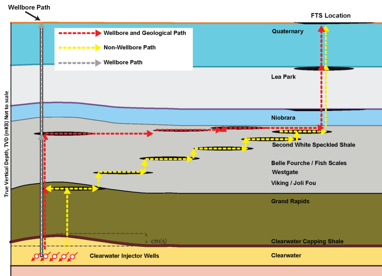
Figure 9-1 Conceptual Flow Path for FTS
