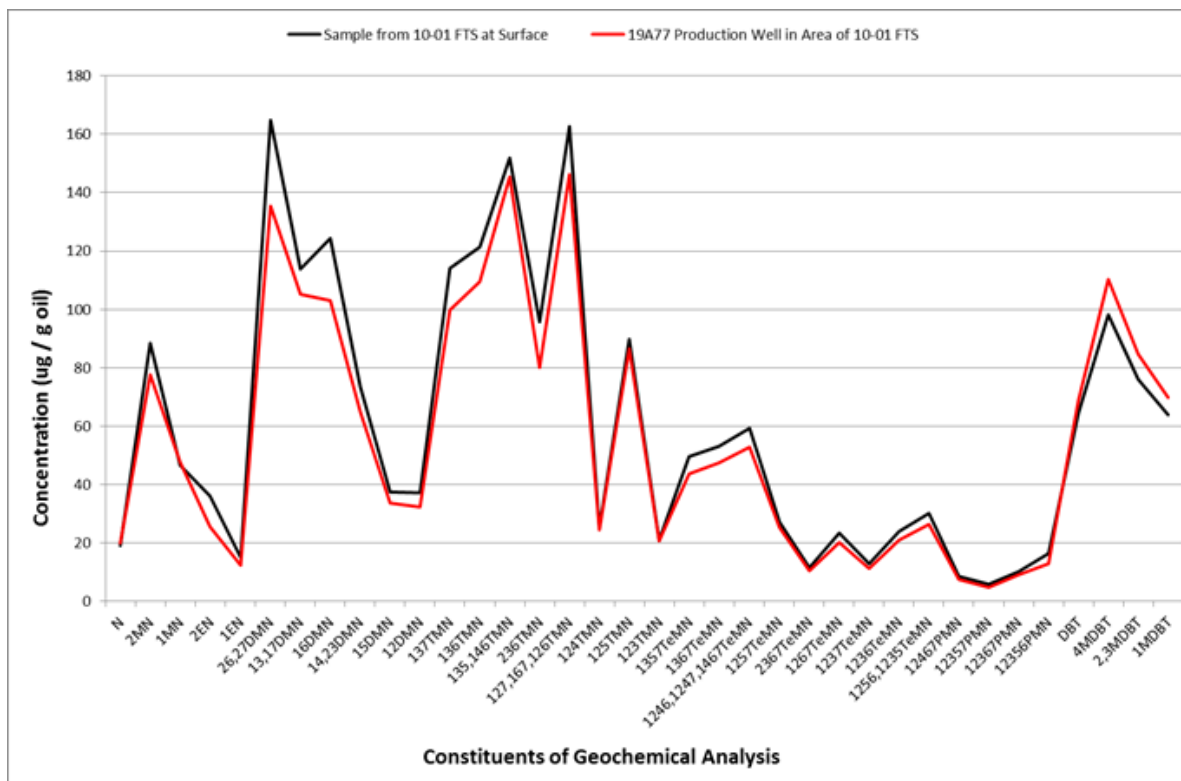
Figure 8-4 10-1 Geochemical Analysis Comparison Plot
