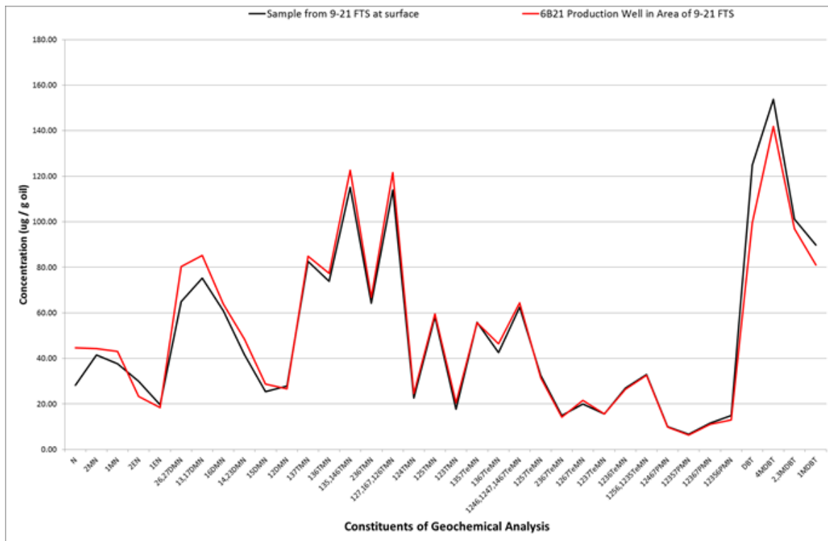
Figure 8-3 9-21 Geochemical Analysis Comparison Plot
