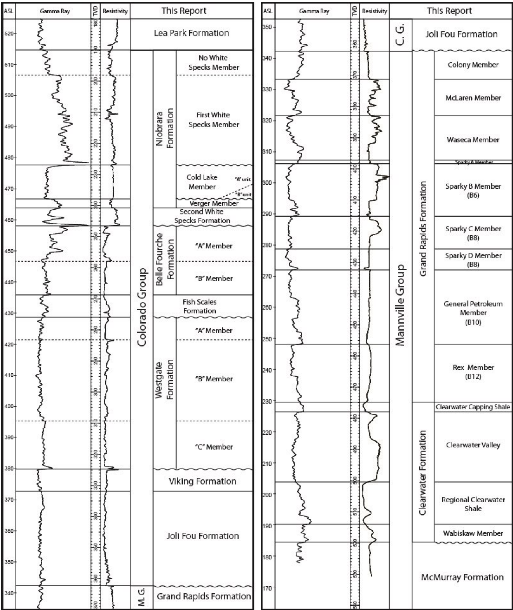
Figure 4-7 Detailed Stratigraphic Column for the Mannville and Colorado Groups in the Primrose Area (Internal Nomenclature)
