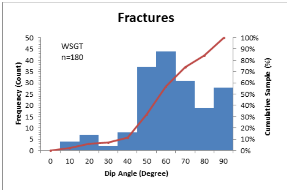
Figure 4-2 Number and Dip Angle of Fractures Observed in the Westgate Formation
