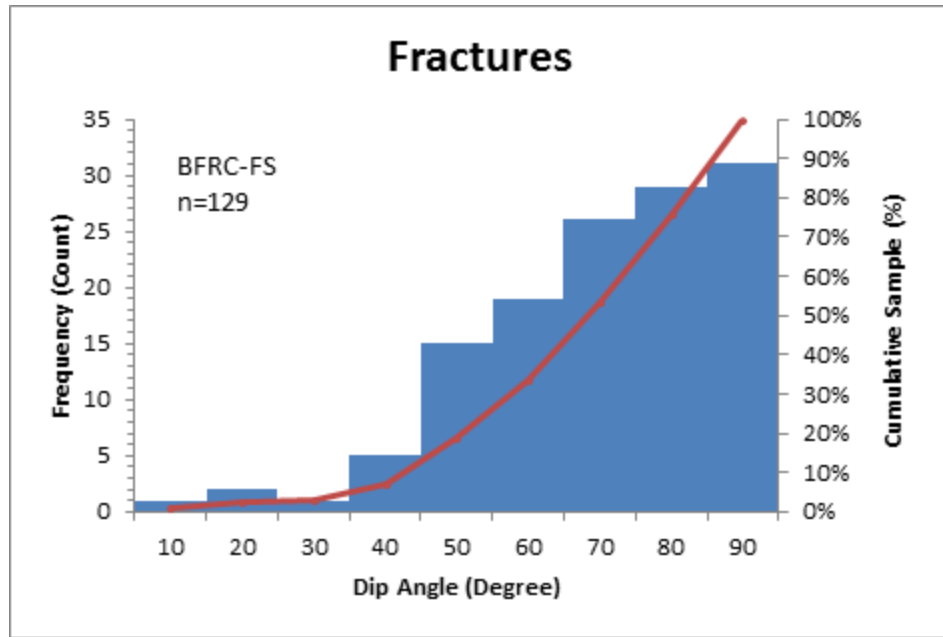
Figure 4-3 Number and Dip Angle of Fractures Observed in the Fish Scales and Belle Fourche Formations
