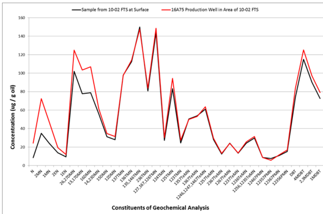
Figure 8-2 10-2 Geochemical Analysis Comparison Plot
