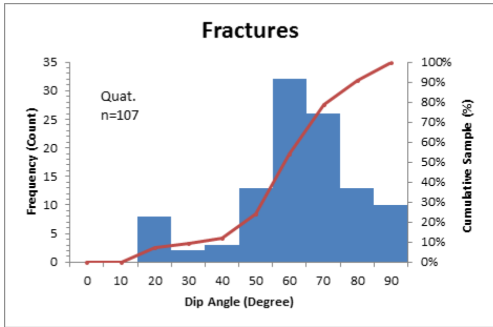
Figure 4-5 Number and Dip Angle of Fractures Observed in the Quaternary Formations
