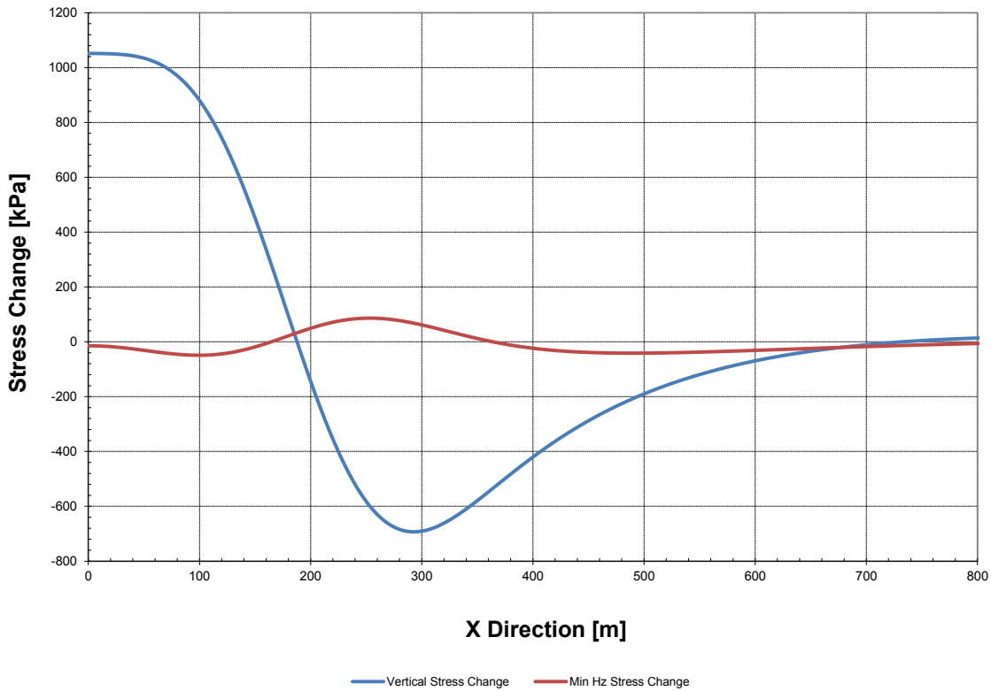
Figure 6-5 Example of total stress changes with distance away from the center of the Clearwater uplift profile at a depth of 360 m
