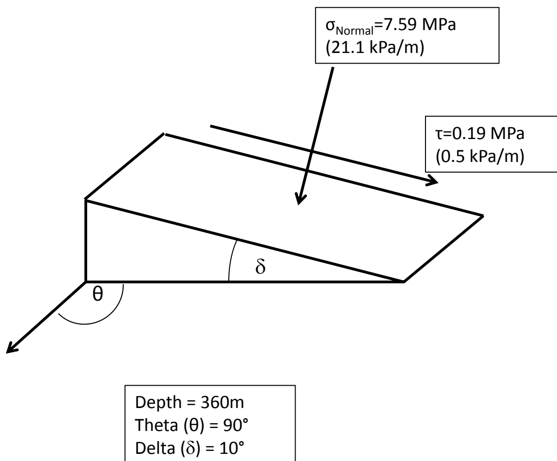
Figure 6-4 Example of stresses acting on a natural fracture with a 10 degree dip at a depth of 360 m
