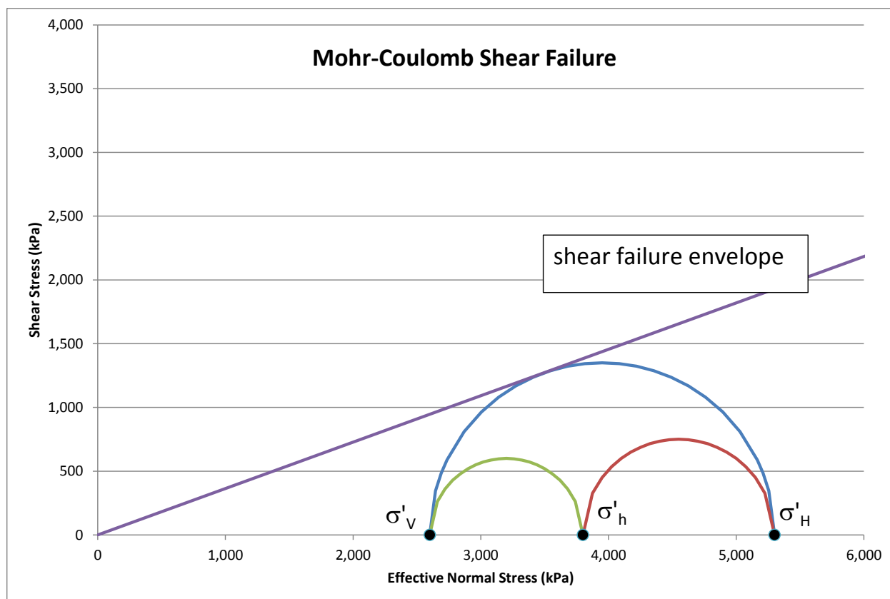
Figure 6-3 A simplified example of shear failure of a natural fracture at a fluid pressure less than the hydraulic fracture pressure
