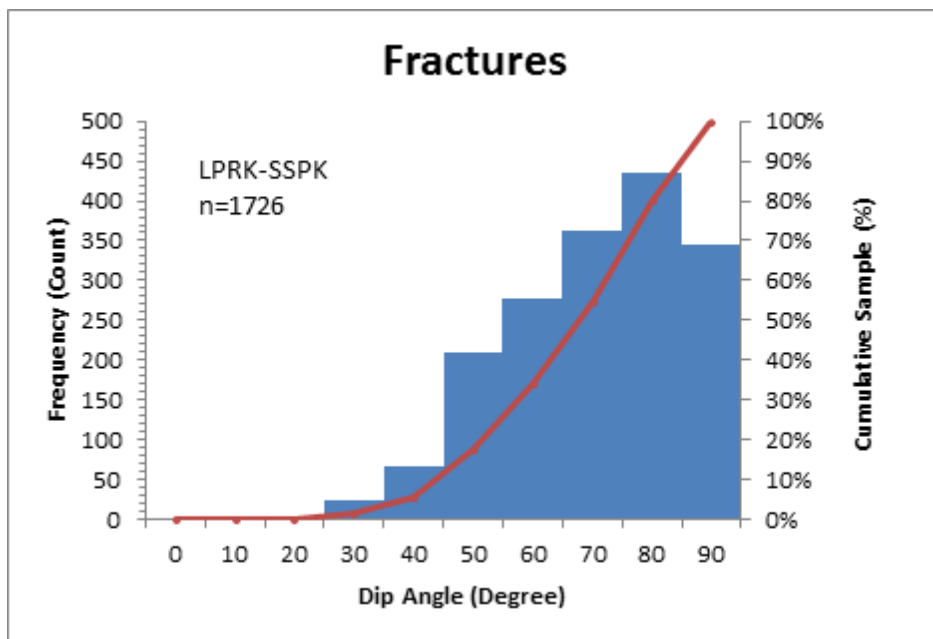
Figure 4-4 Number and Dip Angle of Fractures Observed in the Second White Specks, Niobrara and Lea Park Formations
