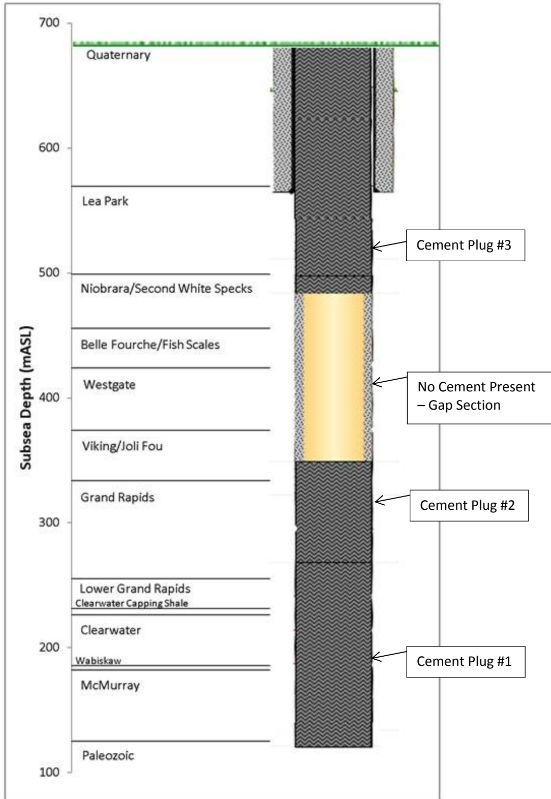
Figure 7-1 Conceptual diagram of the theoretical cement placement for DOME AEC 100/07-22-067-03W4
