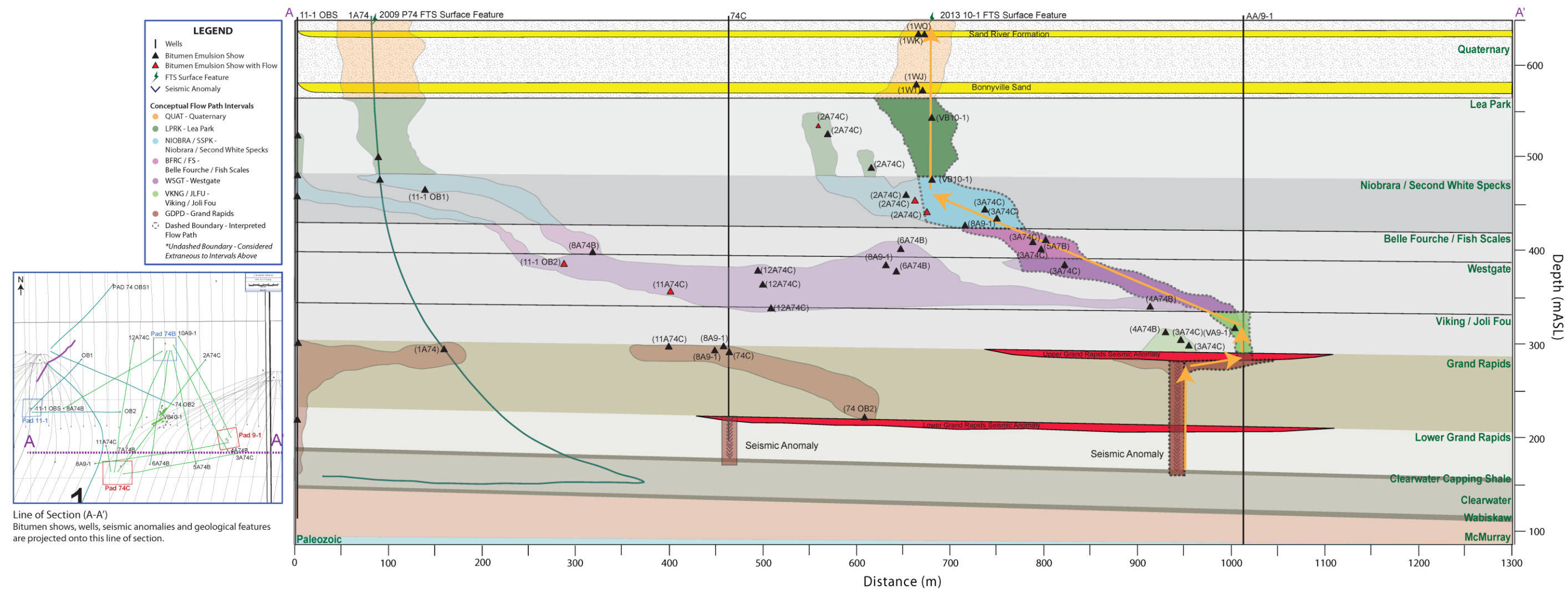
Figure 10-9 10-1 FTS – Features, Data and Conceptual Flow Path Projected on W-E Plane
