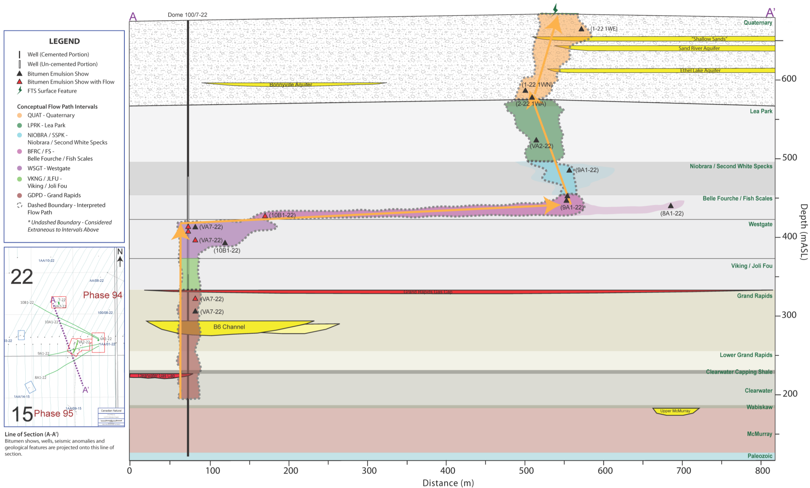
Figure 10-1 2-22 FTS – Features, Data and Conceptual Flow Path Projected on N-S Plane
