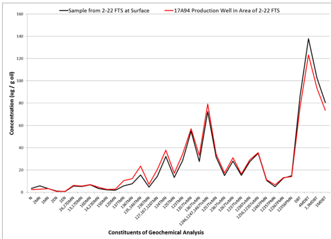
Figure 8-1 2-22 Geochemical Analysis Comparison Plot
