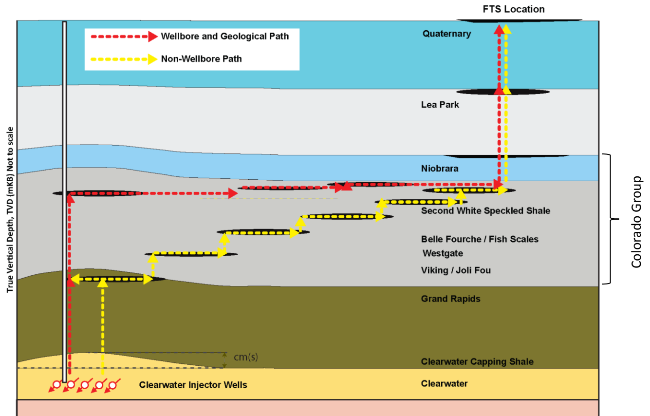
Figure 1-1 Conceptual Schematic of Possible Flow Paths
