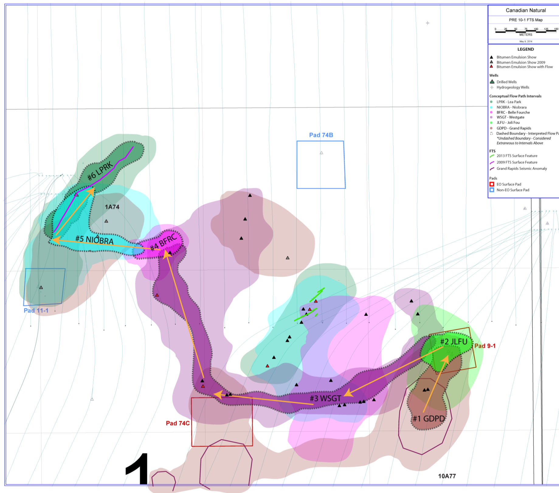
Figure 10-8 Pad 74 FTS – Conceptual Plan View of Bitumen Emulsion Shows
