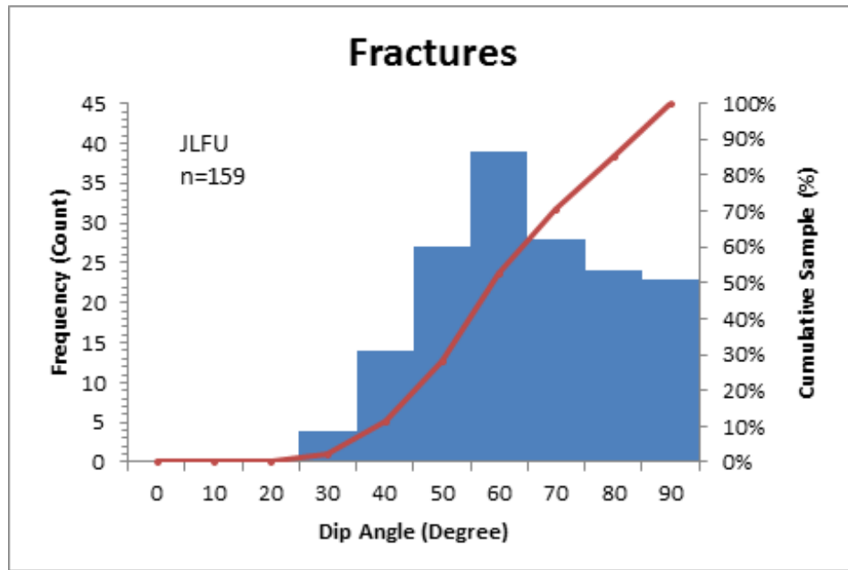
Figure 4-1 Number and Dip Angle of Fractures Observed in the Joli Fou Formation
