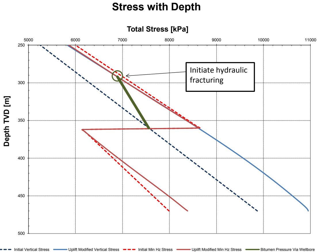
Figure 6-8 Example of stress change with depth and pressure profile along a wellbore path intersecting the minimum stress
