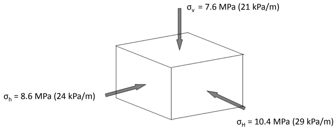
Figure 6-2 Example of Typical Principal Stresses in the Joli Fou Formation at a depth of 360 m
